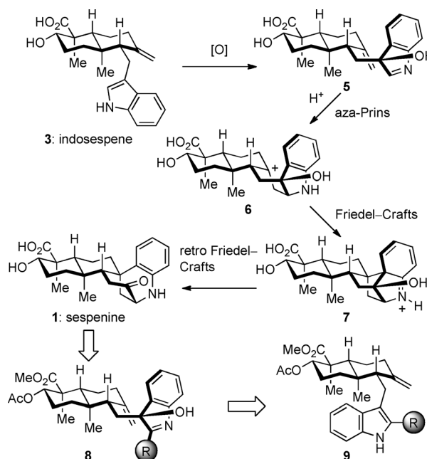
Scheme 1. Retrosynthetic analysis of sespenine based on its postulated biosynthetic model.
