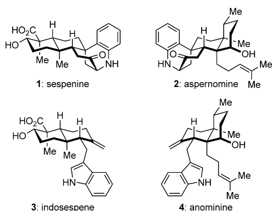
Figure 1. Sespenine and aspernomine, and their plausible biosynthetic precursors indosespene and anominine, respectively.
